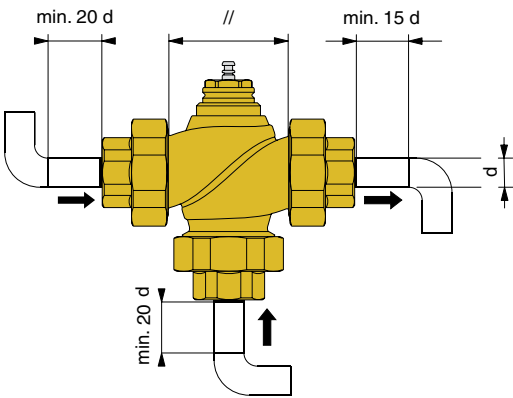
Threaded version
