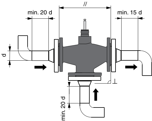
Flanged version
